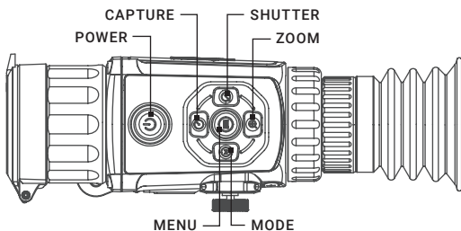
FIGURE 2-2. CONTROL BUTTONS
